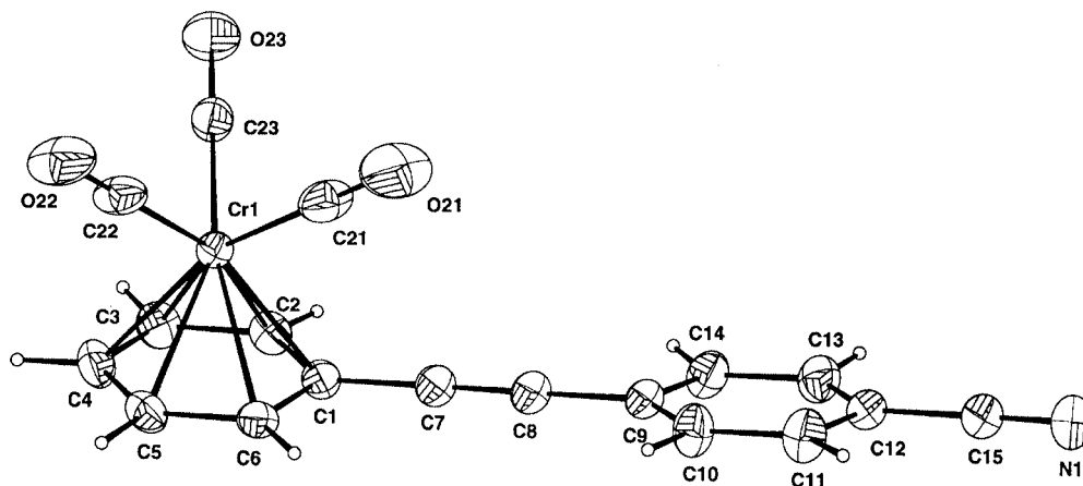
Figure 1. ORTEP diagram and atomic numbering scheme of the molecular structure of complex 1Cr including a view along the Cr–ring axis. Thermal ellipsoids are presented at the 30% probability level
