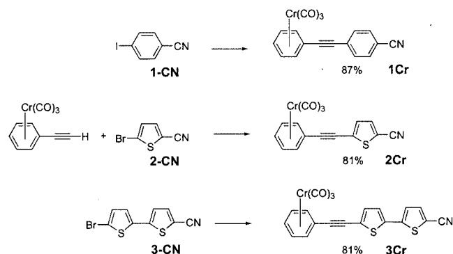
Scheme 1. Sonogashira-coupling reactions
