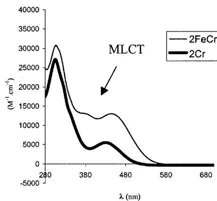
Figure 3. UV/Vis. Electronic spectra of 2FeCr , showing a weak MLCT band, and 2Cr
