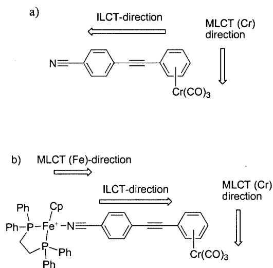
Figure 4. Ground state dipole vectors of chromium mononuclear complexes compared with the corresponding binuclear complexes. The direction of the ILCT contribution in the binuclear complexes is reversed, due to the role of the new ending group [\text{MCp}(\text{DPPE})(\text{N}\equiv\text{C})-]^+
