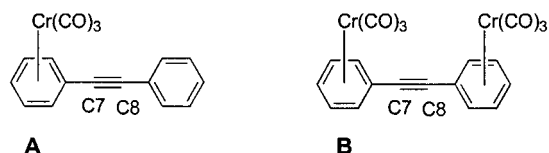
Figure 2. Complexes A [18] and B [19]
